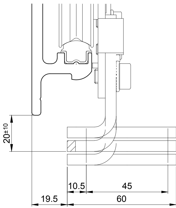
Trolley 2301
